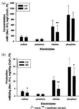
Fig. 1. (a) Electrolyte concentration in urine in control (CN) and ADHD children (AD); and (b) electrolyte production (per kg per day) in control (CN) and ADHD children (AD).
