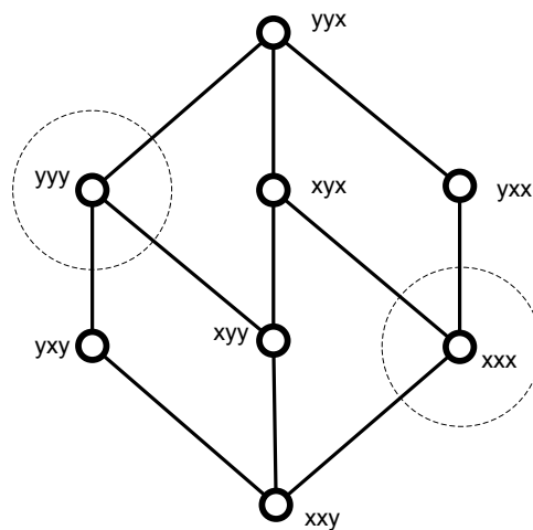
Figure 1 – Volitionality-Intentionality-Rationality Lattice
