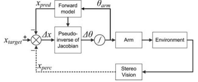
Figure 2: Diagram summarizing our approach of using a learned forward model to incrementally generate reaching trajectory. x_{pred} and x_{perc} stand for the end effector position predicted by the forward model and perceived by the stereo system respectively.
