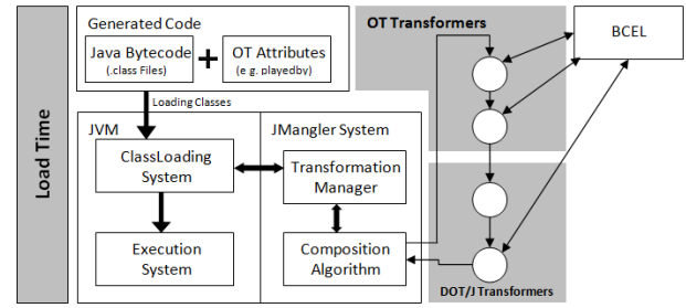
Fig. 3. Integrating DOT/J transformers with OT/J structure.
