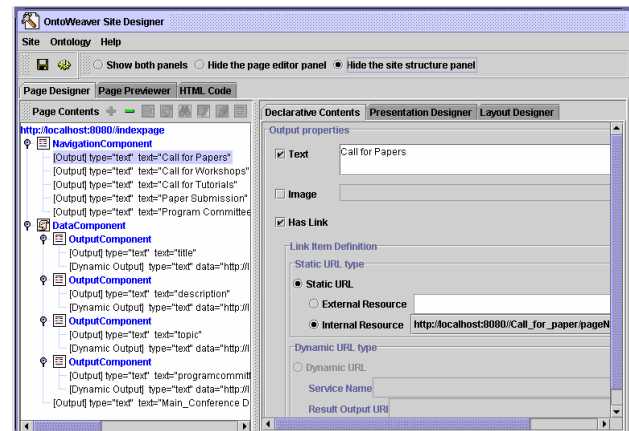
Figure 5 The screenshot of the compositional structure of the index page. The left pane shows the compositional structure of the index page. The right pane shows the content of the selected user interface element.
