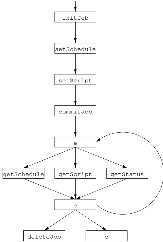
Figure 5: Protocol Graph
