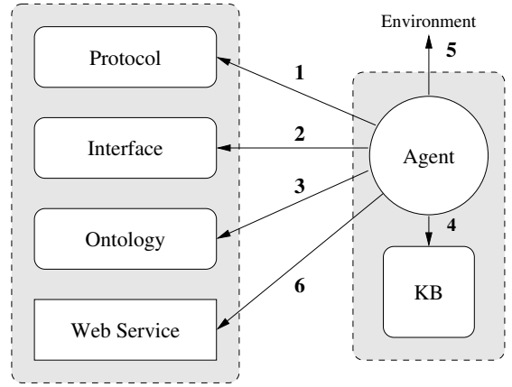
Figure 6: Execution Architecture
