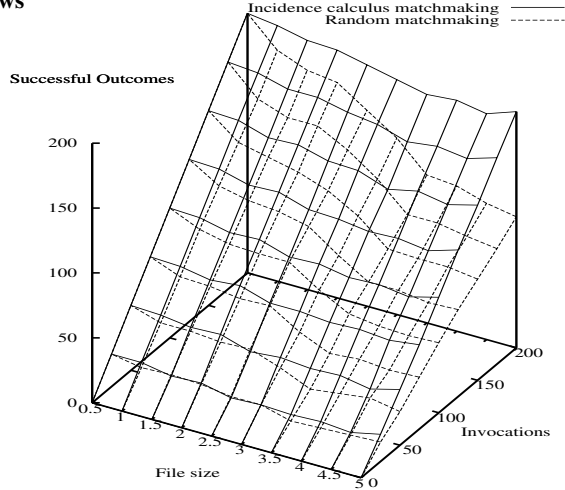
Figure 5: Agent selection improves as matchmaking database grows
