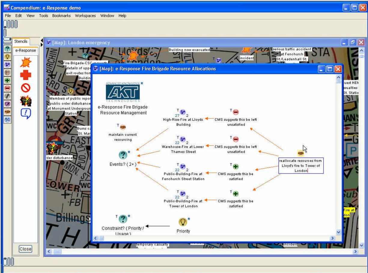
Figure 10. Accepting the CMS resource reallocation.
