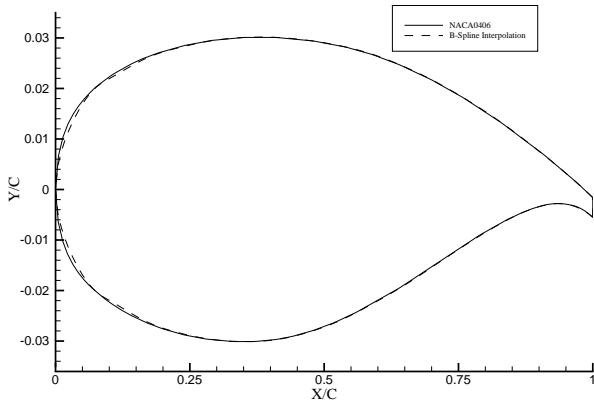
(c) Approximation of geometry to NACA0406 by B-spline interpolation
