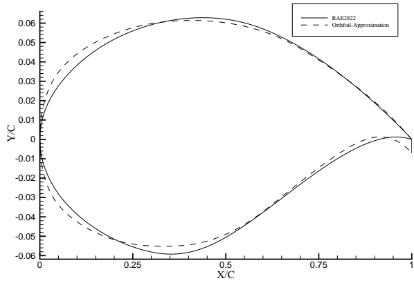
(a) Approximation of geometry to RAE2822 by basis functions approach
