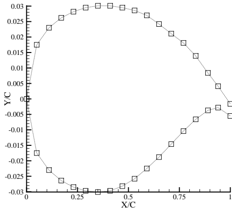
Figure 2. Airfoil Modelling using B-spline interpolation.
