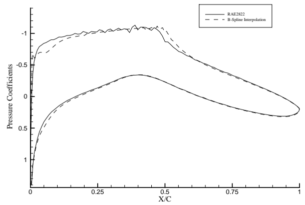
(b) Comparison of pressure distributions for RAE2822 using B-spline interpolation
