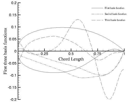
Figure 1. The first three numerically derived orthogonal basis functions.
