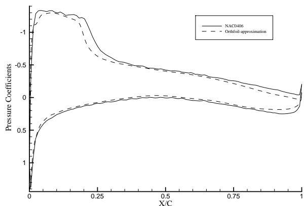
(d) Comparison of pressure distributions for NACA0406 using basis functions
