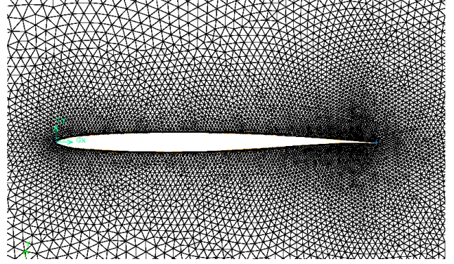
Figure 3. Unstructured mesh used for solving the N-S equations by Fluent
