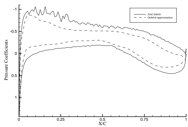
(f) Comparison of pressure distributions for NACA0610 using basis functions
