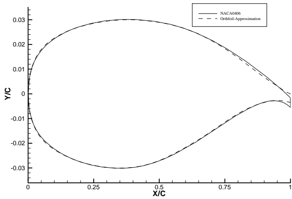
(c) Approximation of geometry to NACA0406 by basis functions approach
