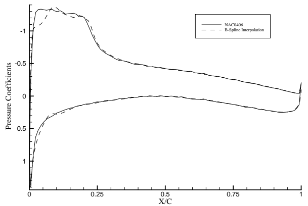
(d) Comparison of pressure distributions for NACA0406 using B-spline interpolation
