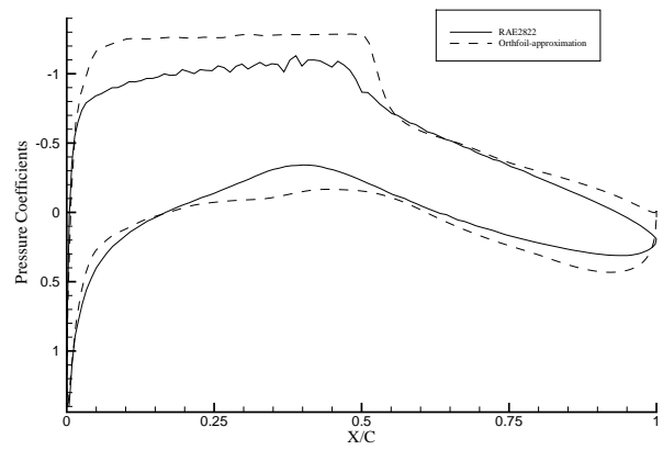
(b) Comparison of pressure distributions for RAE2822 using basis functions
