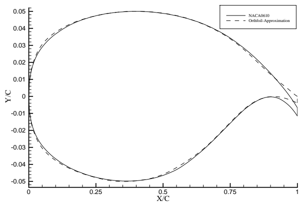
(e) Approximation of geometry to NACA0610 by basis functions approach
