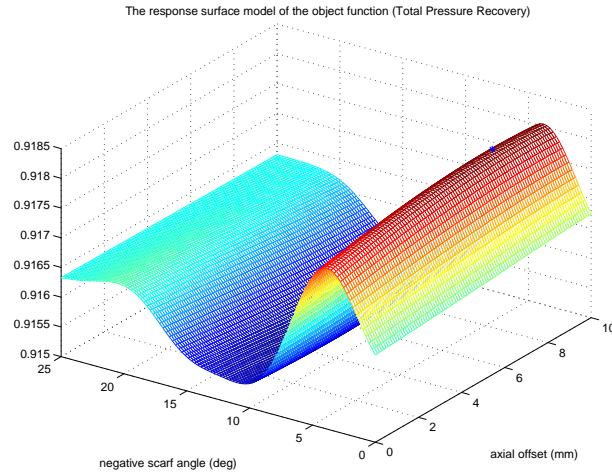
Figure 12. Response surface model of the objective function (Total Pressure Recovery, *: highlighted maximum)
