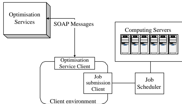
Figure 2. Architecture of Service-Oriented Optimisation System
