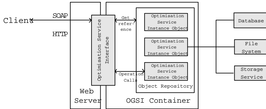
Figure 5. Architecture of the Optimisation Grid Service
