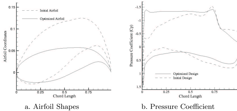
Figure 10. Result of the Airfoil Optimisation
