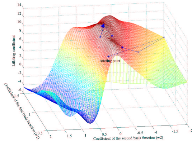
Figure 9. Response surface model and search path for the two-variable airfoil problem with the starting point at w_1 = 0.6 ; w_2 = 0.1815 ; l/d = 9.9238 . Final point found at w_1 = 1.14 ; w_2 = -0.031 ; l/d = 12.2636
