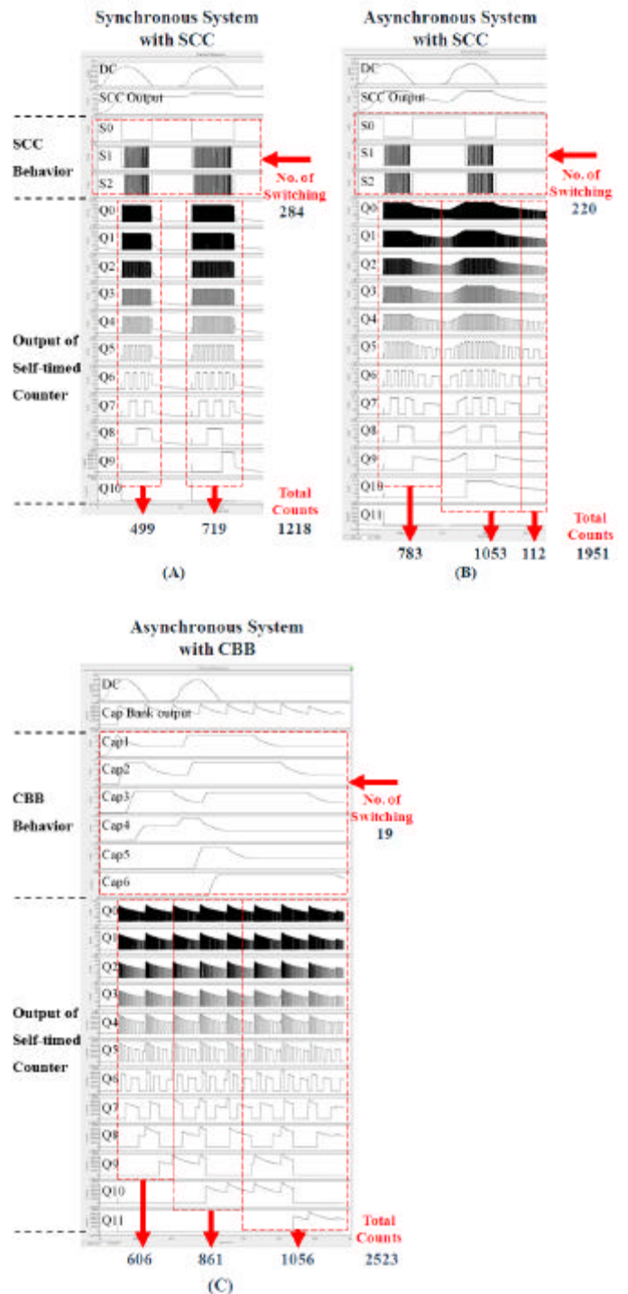
Figure 8. The Counter performances in Terms of Synchronous system with SCC (A), Asynchronous System with SCC (B) and Asynchronous System with CBB (C).
