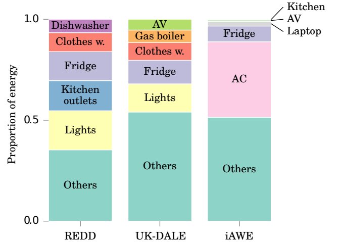
Figure 5: Top five appliances in terms of the proportion of the total energy used in a single house (house 1) in each of REDD (USA), iAWE (India) and UK-DALE.
