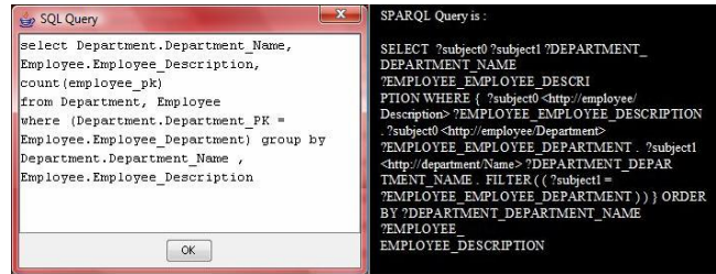
Figure 3: SQL-to-SPARQL Transformation
